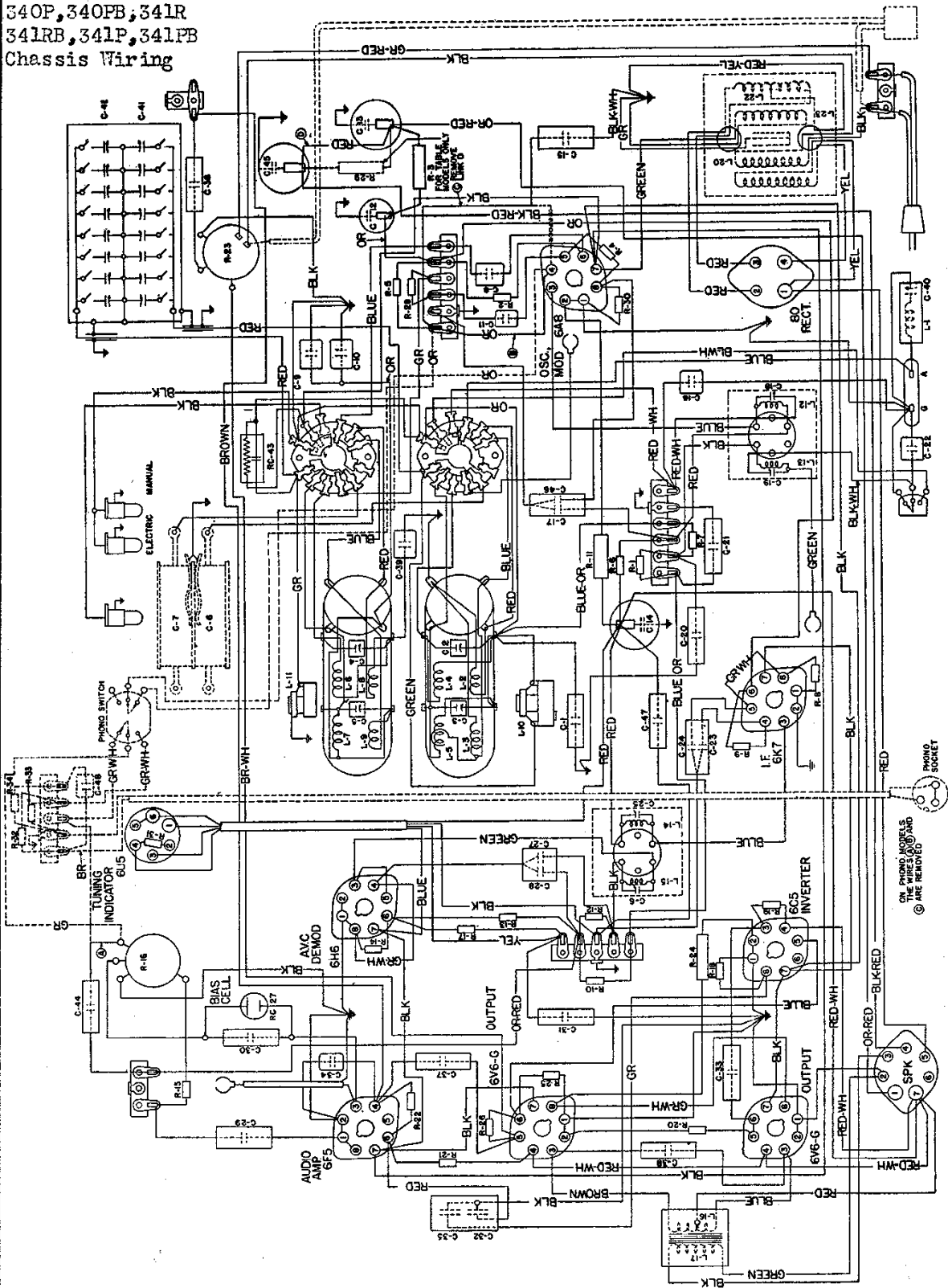
Fig. 3. Wiring Diagram of Chassis.
