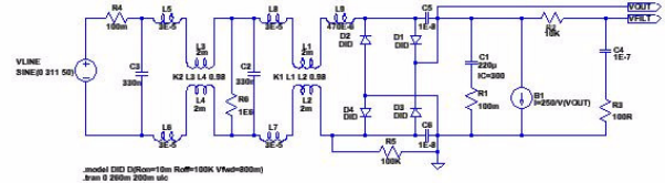
Constant Power 250W DM=470u
