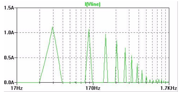
Constant power current spectrum DM=470u
