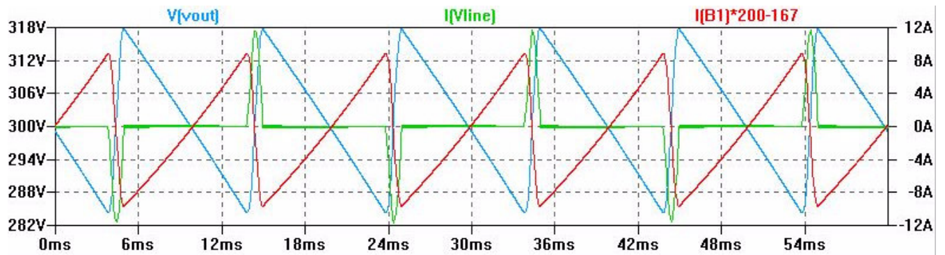
Amplified load current ripple (x200) DM= stray
