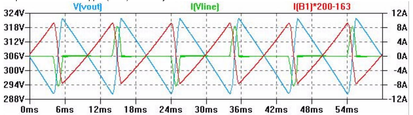
Amplified load current ripple (x200) DM=470u
