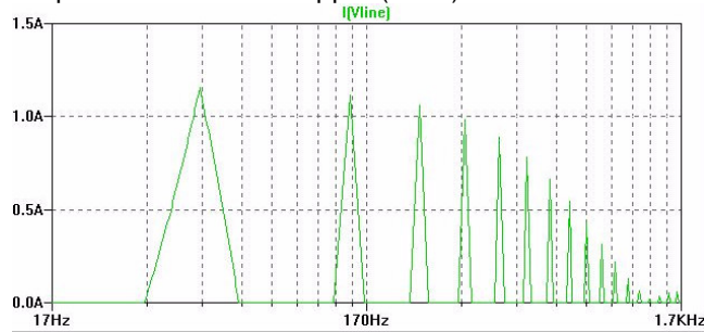
constant power current spectrum DM= stray
