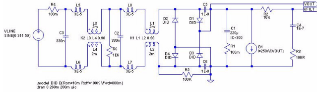
constant power 250W DM= stray
