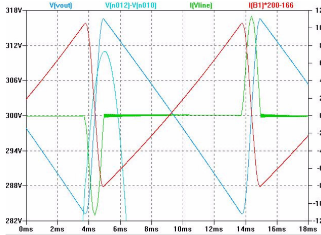
Amplified load current ripple (x200) DM=string
