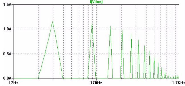
constant power current spectrum DM=string
