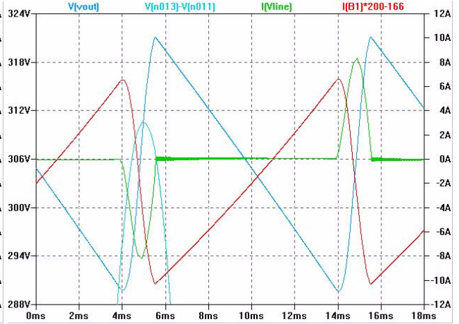
Amplified load current ripple (x200) DM=470u
