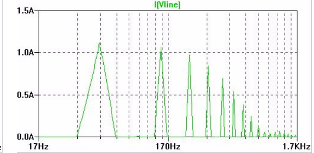
Constant power current spectrum DM=470u
