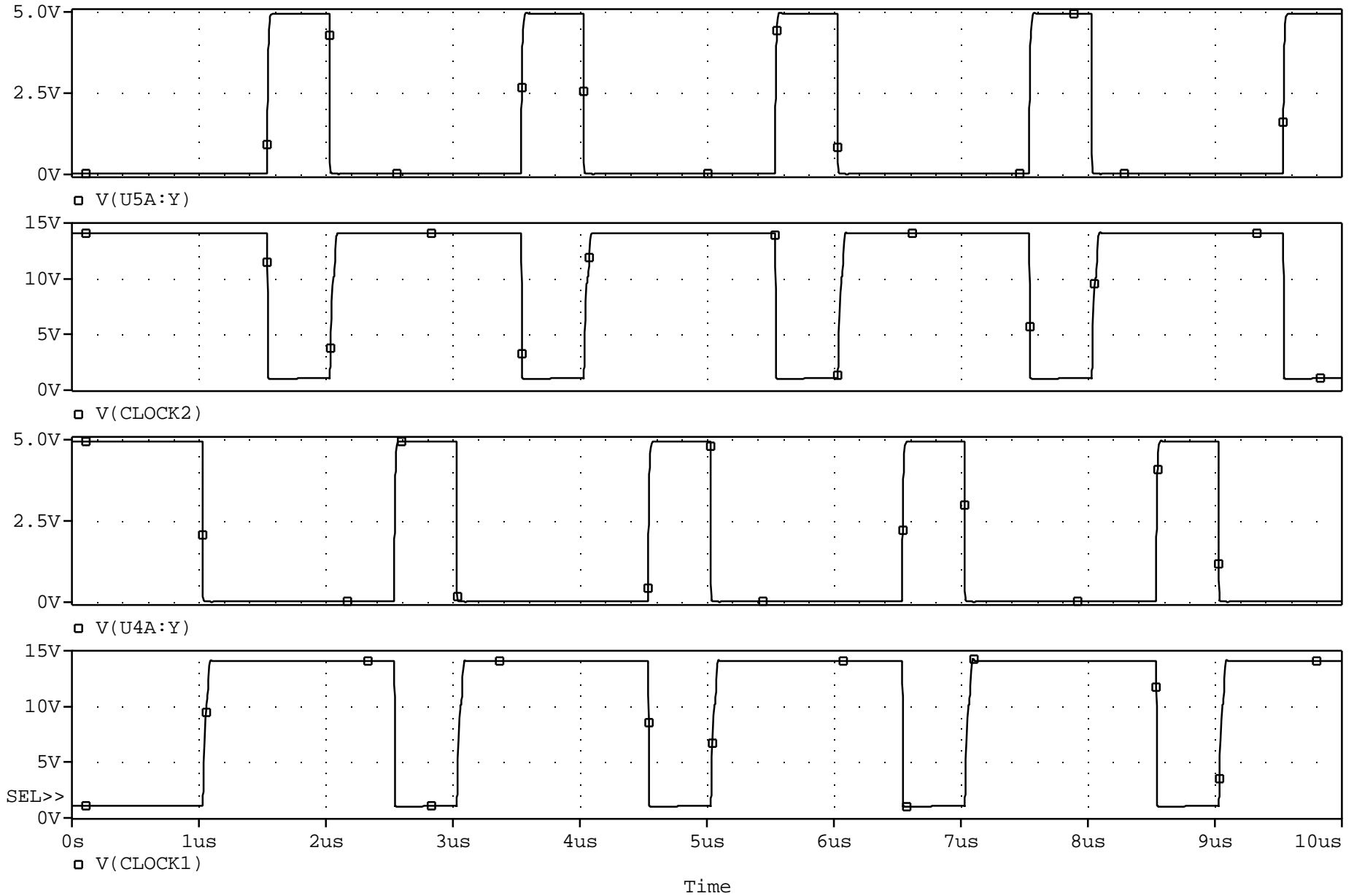
(A) ClockGen with Buffers Made from Discrete Components
